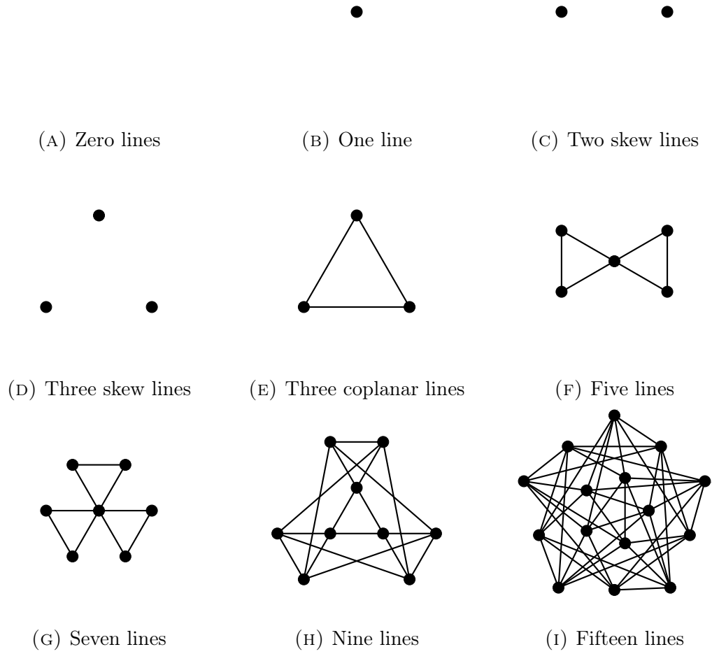
FIGURE 3. Intersection graphs
