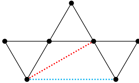
FIGURE 1. Impermissible graph of seven lines
